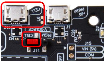
USB power on “CELL” connector
