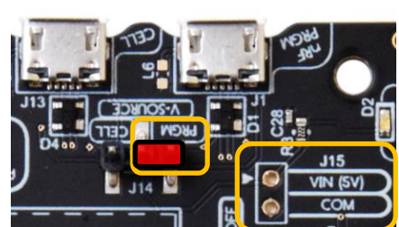
5V power for J15 header
