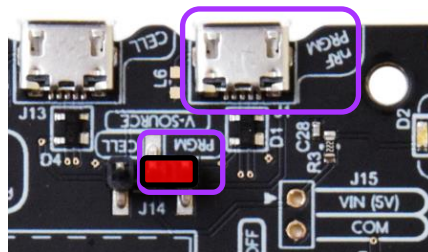
USB power for “nRF PRGM” connector
